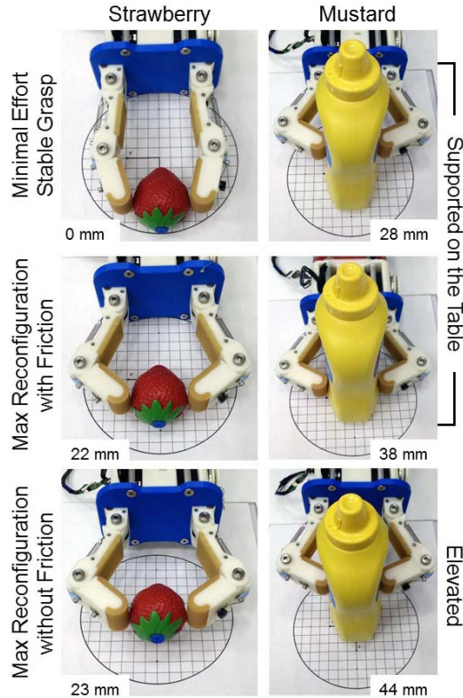
Fig. 17. Symmetric pinch grasps of a lightweight object (plastic strawberry) and a heavy object (bottle of mustard). First row: minimal effort, stable grasps. Second and third rows: maximum reconfiguration poses with friction (the object lies on the table) and without friction (the object is elevated). White boxes contain the values of the magnitude of reconfiguration.
