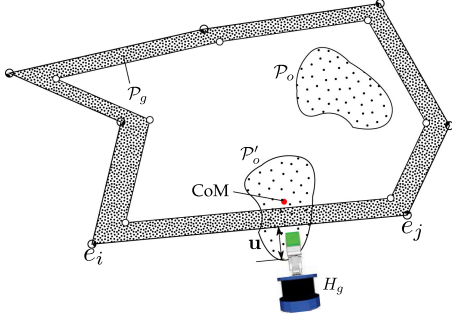
Fig. 5. A support surface is represented as a polygon with edge points Q = (e_1, \dots, e_{n_s}) . P_g is a set of points near the surface edges. An object represented by point cloud P_o is slid to P'_o located near one of the surface edges. u is the largest distance between the edge (e_i, e_j) and object's points which stick out of support surface. The object can be grasped using the hand pose H_g if u is large enough.
