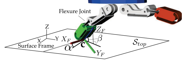
Fig. 4. A fingertip is in contact with the top surface of an object at c \in \mathcal{P}_o . The X_F -axis (red) of the fingertip frame is always aligned in the X - Y plane of \mathcal{S}_{top} . The angle \alpha represents the yaw rotation of X_F -axis about the surface normal. \beta is the pitch angle between the Z_F -axis (blue) of the fingertip frame and the object surface.
