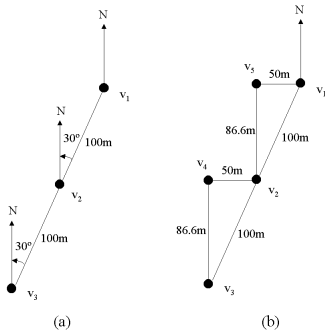
Fig. 1. Line Formation (a) Heading Determined Formation (b) Equivalent Distance Determined Formation
