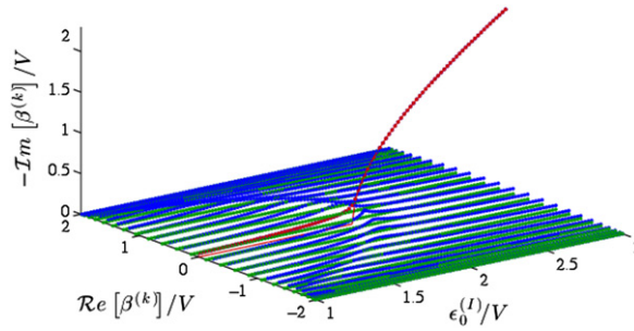
Figure 1. Parametric evolution of the propagation constants \beta^{(k)} of an array of N = 49 coupled waveguides with one dissipative ( \epsilon_0^{(I)} > 0 ) defect in the middle, as a function of \epsilon_0^{(I)} . The phase transition occurs at \epsilon_0^{(I)} = \epsilon_{cr}^{(I)} \equiv +2V where the defect mode profile (shown as red dots) switches from non-exponential to exponential decay. The solid red line shows the asymptotic analytical result, equation (5). Similar behavior (not shown here) but with the \beta 's in the upper complex plane can be observed for gain \epsilon_0^{(I)} < 0 where \epsilon_{cr}^{(I)} = -2V . The green lines indicate modes with real propagation constants which are solutions of the first equation (11). In the case of even number N they also acquire an imaginary part in the propagation constant, similar to the modes shown in blue.
