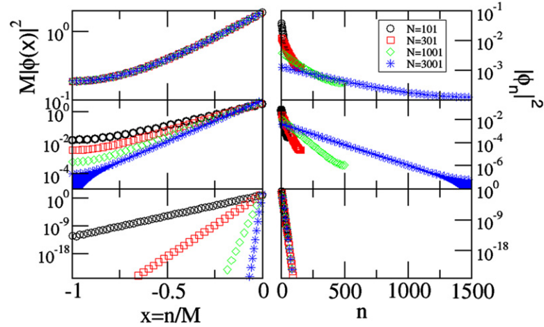
Figure 2. FB defect mode for various system sizes N = 2M + 1 . Left panels report the left part ( n < 0 ) of these modes (the right part n > 0 is the same) by employing the scaling M\phi(x = n/M) while the right panels report the right part n > 0 of these modes without any scaling. In the former representation an extended state is invariant under increase of the size of the system while in the latter, the scale invariance is demonstrated for localized modes. Three defect values of \epsilon_0^{(I)} have been used: (upper) 0 < \epsilon_0^{(I)} = 1.9 \text{ V} < 2 \text{ V} where the mode is delocalized; (middle) \epsilon_0^{(I)} = 2 \text{ V} where the mode is critical; (lower) \epsilon_0^{(I)} = 2.1 \text{ V} > 2 \text{ V} where the mode is exponentially localized.
