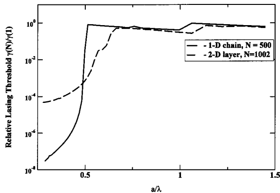
Fig. 6. Relative lasing threshold for finite chain and planar layers of resonant dipoles [ \gamma(1) is the single-particle decay rate].
