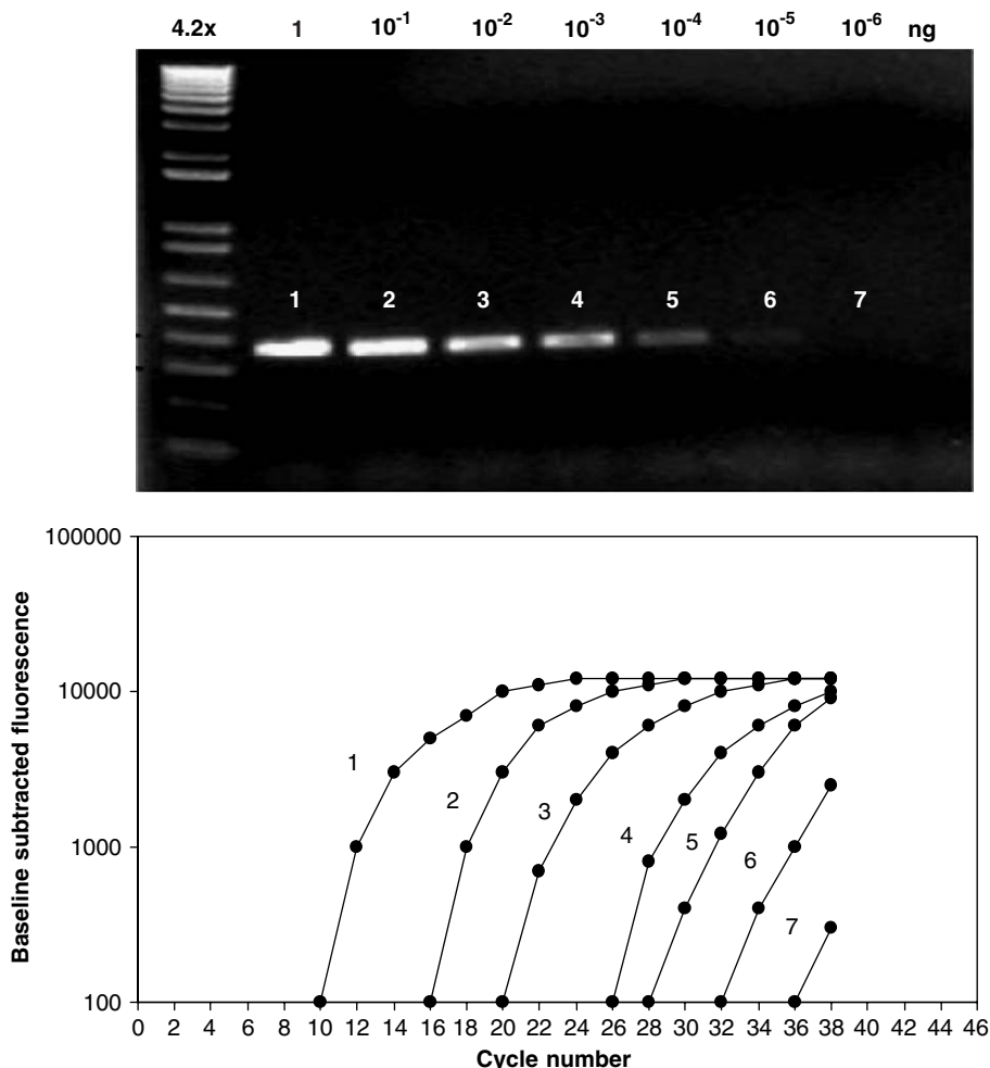
Fig. 3. A dilution series demonstrating detection sensitivity and the quantitative PCR method. The electrophoresis gel represents conventional PCR while the graph below represents \log_{10} fluorescence versus time for real-time PCR. Figure adapted from Zeng et al. (2004).
