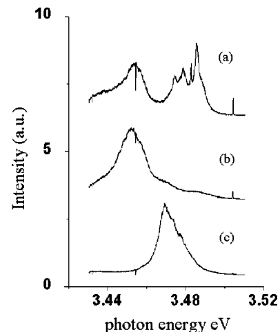
FIG. 3. These three spectra from separate points along the IDB illustrate the spectral inhomogeneity of the boundary emission. Narrow features, like those in (a), are observed intermittently. Typical IDB spectra look most like (b) and are centered 30–40 meV below the peak emission energies of bulk GaN with Ga-face polarity.
